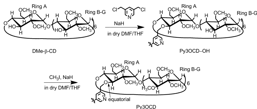
Scheme 2. Synthesis of Py3OCD. DMF = dimethylformamide, THF = tetrahydrofuran.
